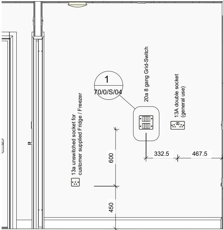
B Kitchen Electrics - View B 1 : 25
