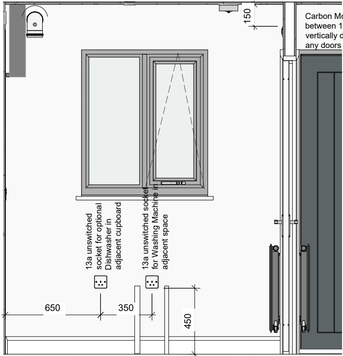
A Kitchen Electrics - View A 1 : 25
