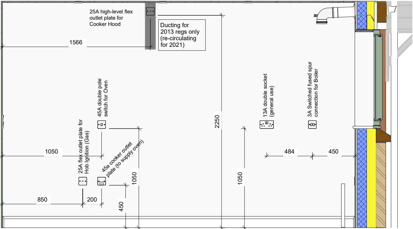
C Kitchen Electrics - View C 1 : 25
